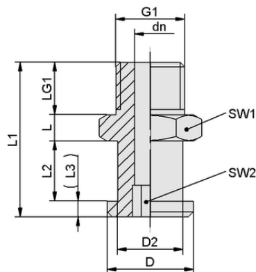
Design data SA-NIP N011 G1/4-AG DN350
