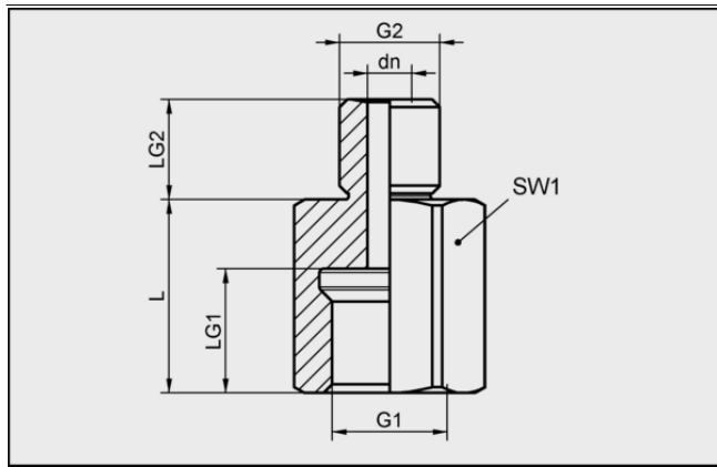
Design data SA-NIP N009 G1/4-IG DN440
