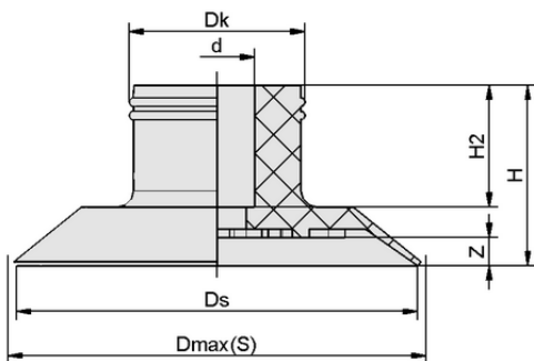
Design data SGP 24 HT1-60 N016
