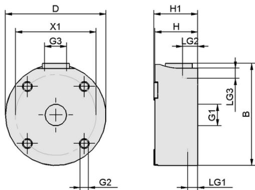
Design data SBS 40 HF G1/8-IG AL
