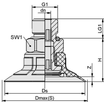
Design data SPF 50 ED-65 G1/4-AG
