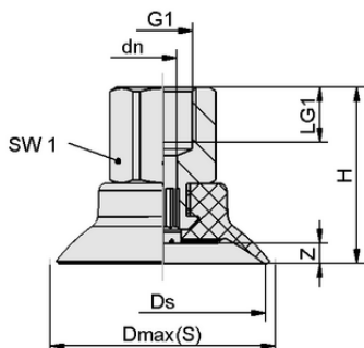
Design data SUF 30 SI-55 G1/8-IG
