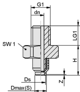
Design data SUF 1 NBR-ESD-55 M3-AG
