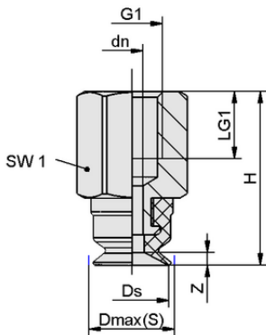
Design data SUF 6 NBR-55 M5-IG
