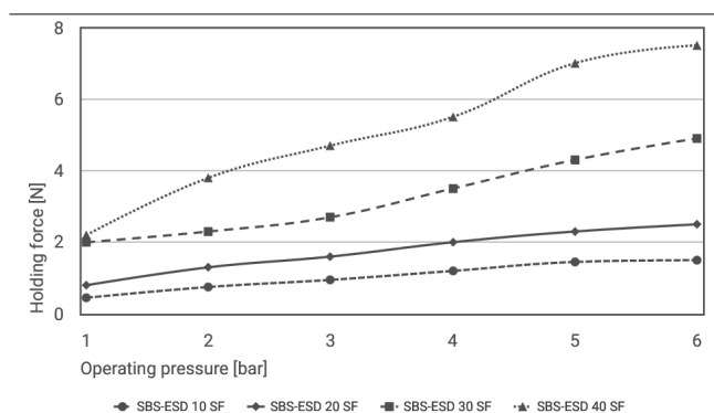
Holding force
