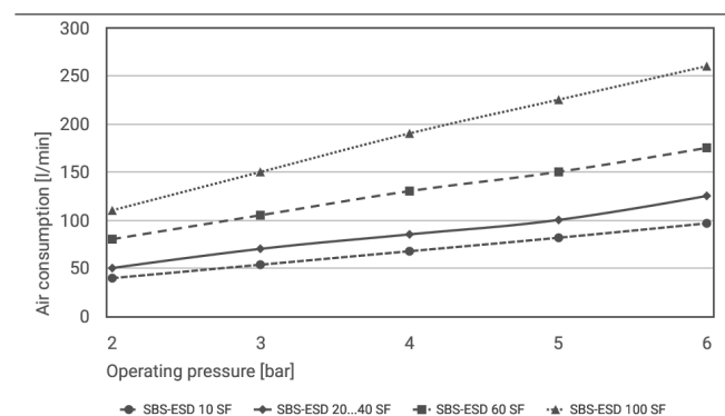
Air consumption
