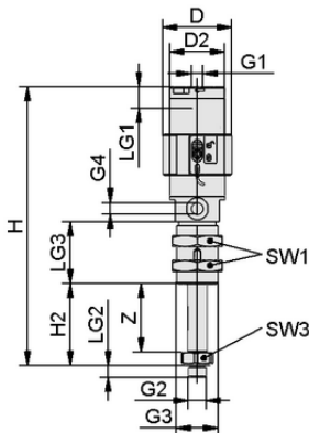
Design data FST-LOCK-HD G1/4-AG 50 NC VG SFP
