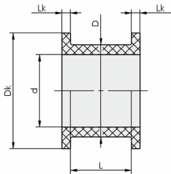
Design data BUCHSE 32-25x21 PA
