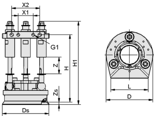
Design data DBD 130x187 80 M54
