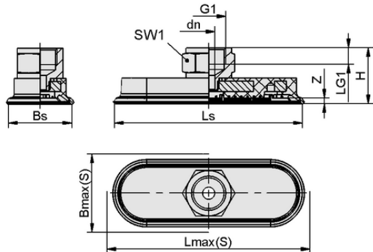
Design data SAOF 90x30 HT2-65 G3/8-IG
