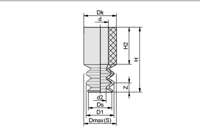
Design data FG 5 SI-55 N017
