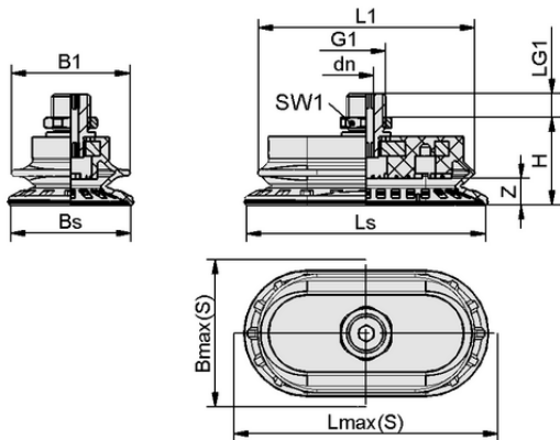
Design data SAOB 60x30 HT2-65 G1/4-AG
