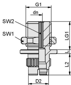
Design data SC-A 055-AR G1/4-AG L
