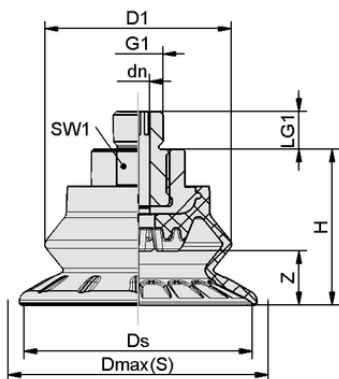
Design data SAB 60 HT2-65 G1/4-AG
