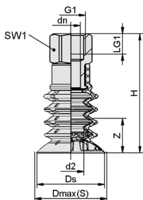
Design data SPB4f 30 SI-55 G3/8-IG
