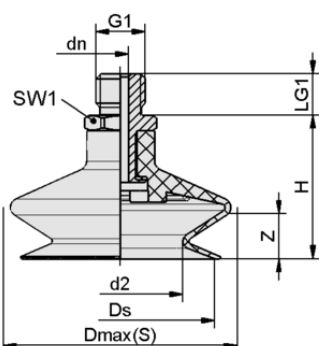
Design data FSGA 16 SI-MD-55 M5-AG
