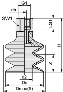
Design data FSG 20 NBR-ESD-55 G1/8-IG
