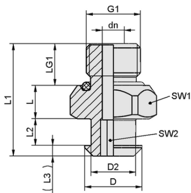
Design data SC 050 G1/4-AG SW410
