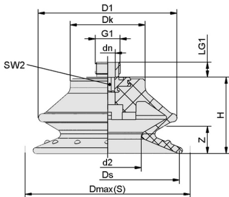
Design data SDC1 100 PU 30/60 G3/8-AG
