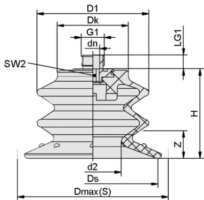
Design data SDC2 75 PU 30/60 G3/8-AG
