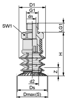
Design data PSPF 33 SI-30/55 G3/8-AG
