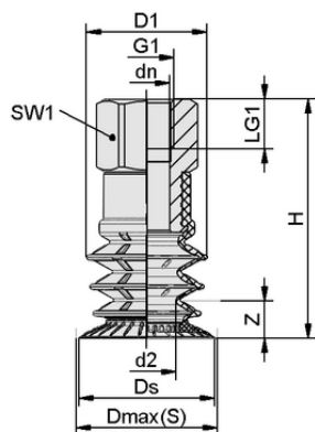
Design data PSPF 53 SI-30/55 G1/4-IG
