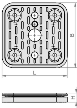
Design data VCSP-O 120x120x16.5 TPE
