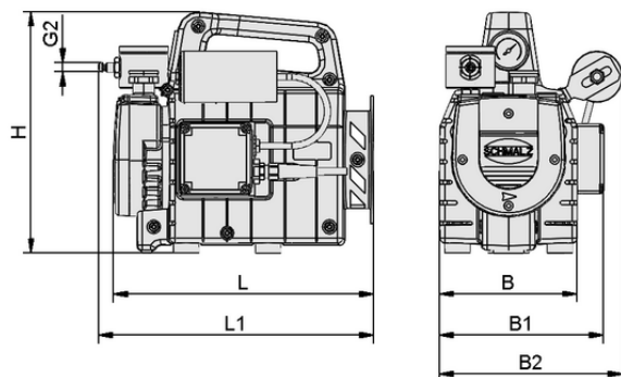
Design data VC-M-PU 4 110V-AC
