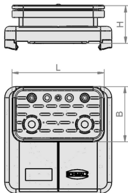
Design data VCBL-S4 130x30x50 TV
