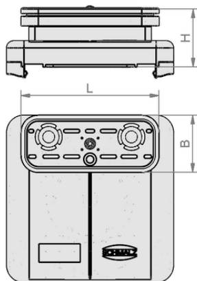
Design data VCBL-S1 120x50x32.7 TV-S
