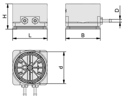
Design data ISMB-G 80x80x55
