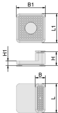
Design data ISBL-HD 80x40x38
