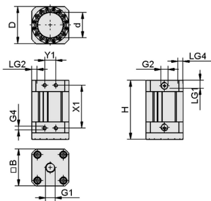
Design data SGM 30 G1/8-IG
