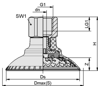
Design data SAXM 40 ED-85 G3/8-IG
