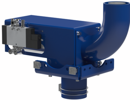
VENT-BGR EMVP-75 3/2 NO 24V-DC
