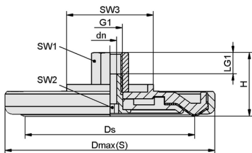
Design data SPL-HT 90 ST G1/4-IG
