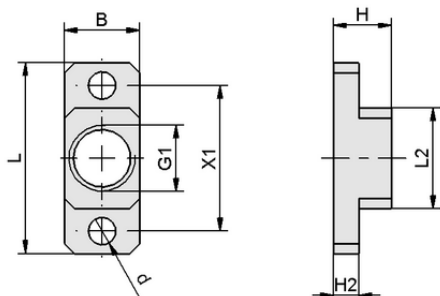
Design data BEF-PL 38x15x11.5 G1/4-IG SNG
