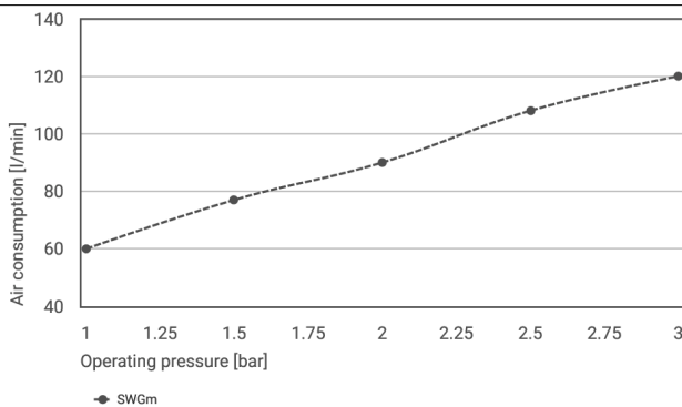
Air consumption
