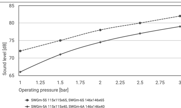
Sound level "free suction" at various operating pressures
