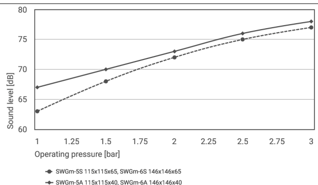
Sound level workpiece gripped at various operating pressures
