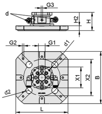
Design data SWGm-5A 115x115x40 1xE100 A PEEK
