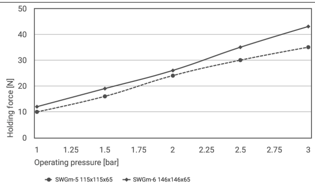
Holding force
