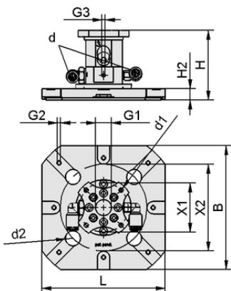
Design data SWGm-5S W 115x115x65 PEEK
