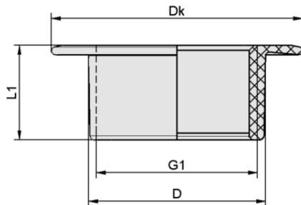
Design data VEE-PL G1/4-IG
