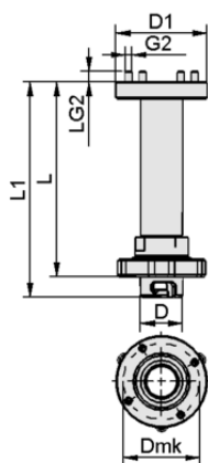
Design data VEE-FE 25.4x131.5
