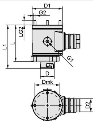
Design data VEE-RU 55x83.5 60 QCM
