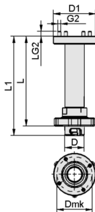
Design data VEE-FE 25.4x81.5
