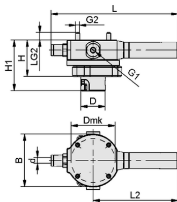
Design data VEE-QCMV HV 2 07 13 SD
