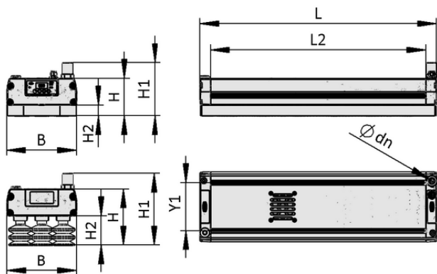
Design data FA-Xi SVK 442 3R18 O20
