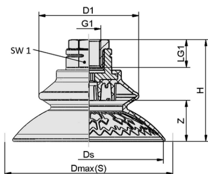
Design data SAXB 100 ED-85 G1/4-IG
