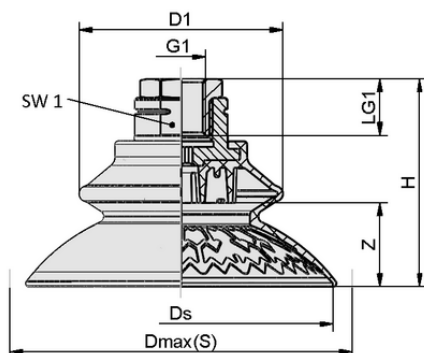
Design data SAXB 120 ED-85 G1/4-IG
