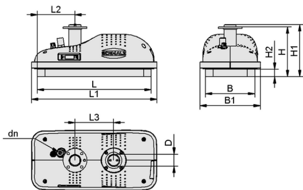
Design data FMCB-SW110 300 3R18 O20 VSi
