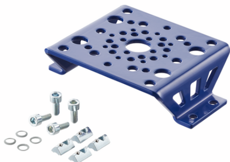
MOD-FLAN 152x109 FXP/FMP-60
