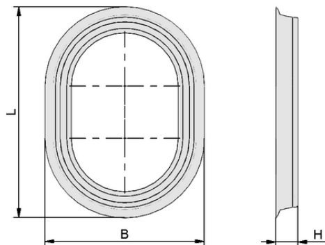
Design data DR-PSSG 350x250 SI-55
