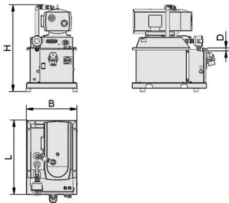
Design data VH-TR Plus 25 30
